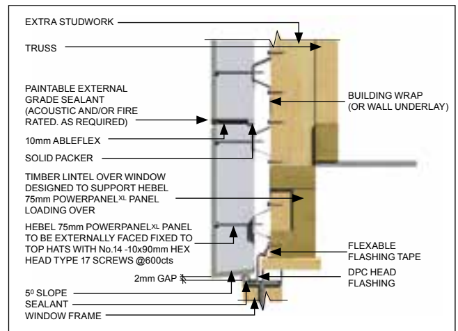
Detail 3.32 – Gable end wall detail – lintel panel over window
